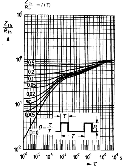
Permissible pulse load \frac{Z_{th}}{R_{th}} = f(\tau)
