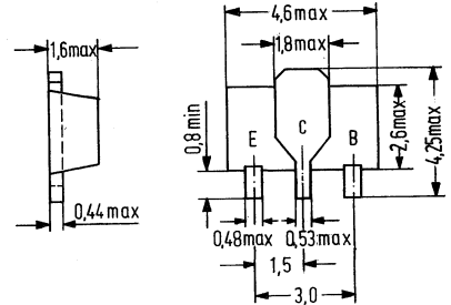
Approx. weight 0.1 g Dimensions in mm
