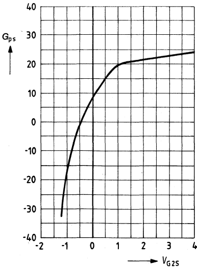
Power gain G_{ps} = f(V_{G2S}) V_{DS} = 15\text{ V} ; V_{G1S} = 0 I_{DSS} = 10\text{ mA} ; f = 200\text{ MHz} (see figure 1)
