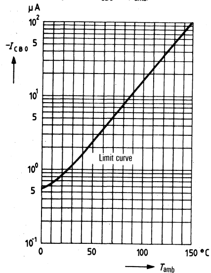
Collector cutoff current versus temperature I_{CBO} = f(T_{amb})
