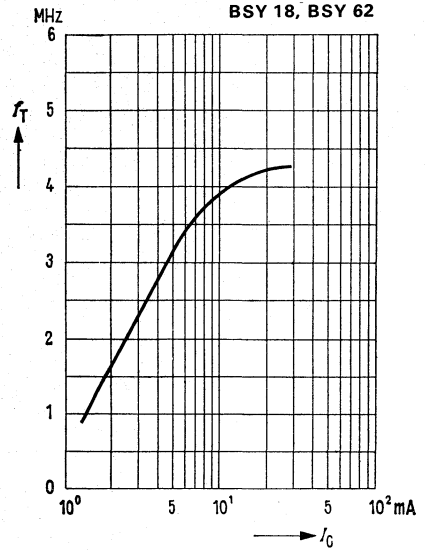
Transition frequency f_T = f(I_C) V_{CE} = 10\text{ V}; f = 100\text{ MHz}; T_{\text{amb}} = 25^\circ\text{C}
