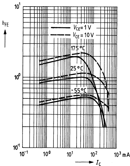
DC current gain h_{FE} = f(I_C) V_{CE} = 1 \text{ V}, V_{CE} = 10 \text{ V}; T_{amb} = 25^\circ \text{C}
