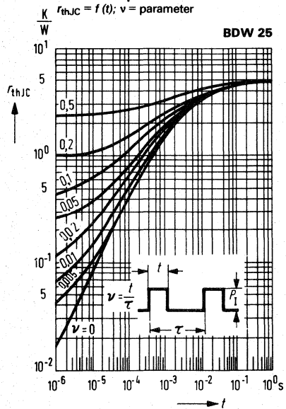
Permissible pulse load
