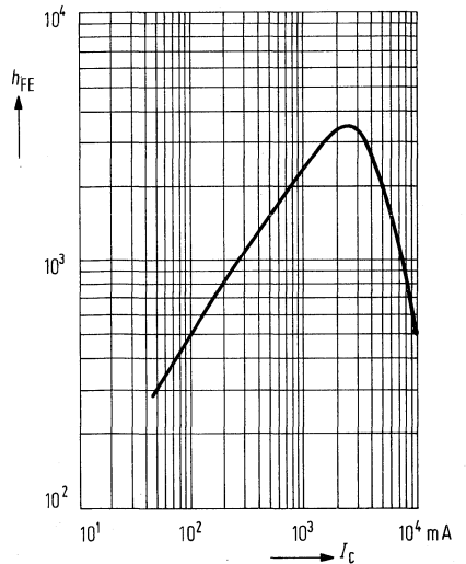
DC current gain h_{FE} = f(I_C) V_{CE} = 3V; T_{case} = 25^{\circ}C BD 643, BD 645, BD 647, BD 649
