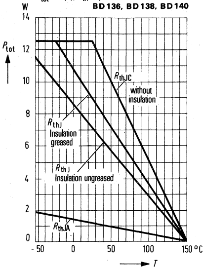
Total perm. power dissipation versus temperature P_{tot} = f(T); R_{th} = \text{parameter} BD 136, BD 138, BD 140
