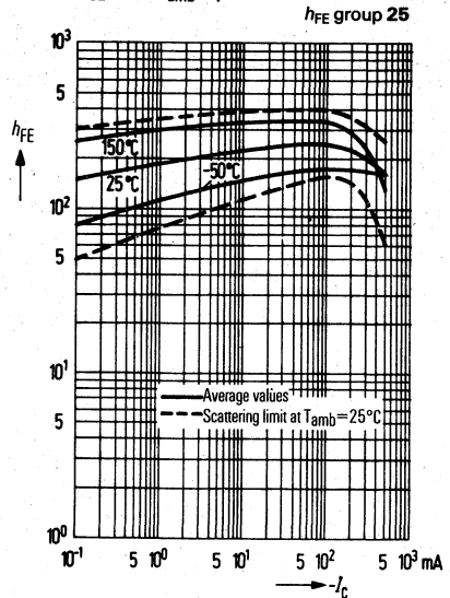
DC current gain h_{FE} = f(I_C) V_{CE} = 1 \text{ V}; T_{amb} = \text{parameter}
