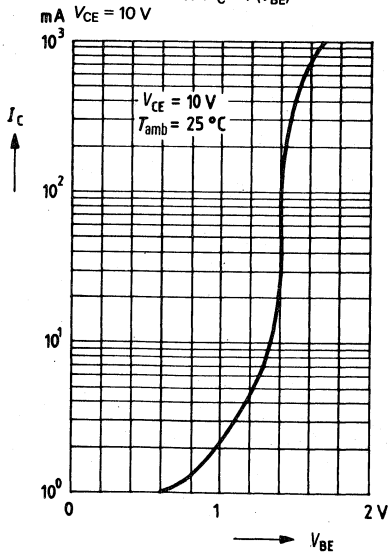
Collector current I_C = f(V_{BE})
