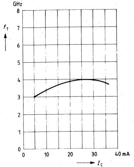
Transition frequency f_T = f(I_C) V_{CE} = 10\text{ V}
