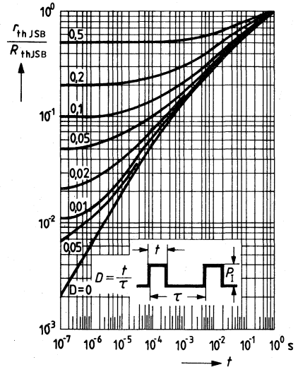
Perm. pulse load \frac{r_{thJSB}}{R_{thJSB}} = f(t) D = parameter
