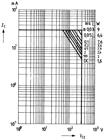
Permissible operating range I_C = f(V_{CE}) T_{case} \leq 110^\circ\text{C} , d = 0.01
