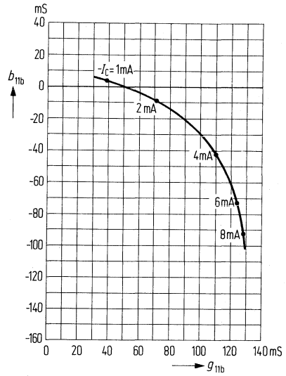
Input admittance Y_{11b} (common base configuration) f = 100 \text{ MHz}; -V_{CE} = 10 \text{ V}
