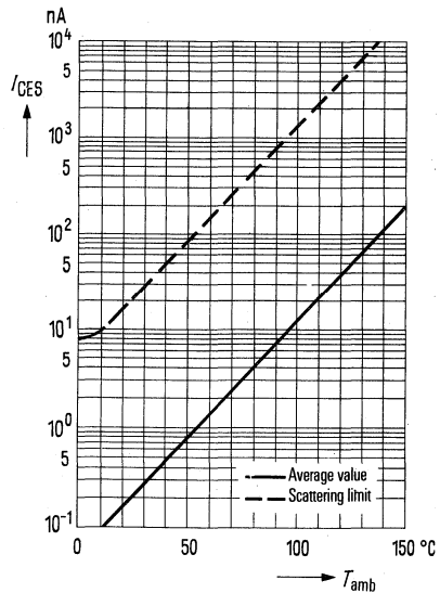
Collector cutoff current versus temperature I_{CES} = f(T_{amb}) for max. permissible reverse voltage
