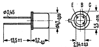
Approx. weight 0.3 g Dimensions in mm
