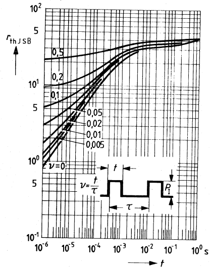
Permissible pulse load r_{thJSB} = f(t) v = \text{parameter}
