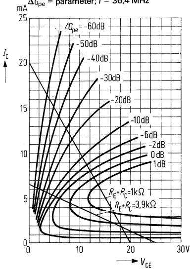
Constant power gain characteristics
