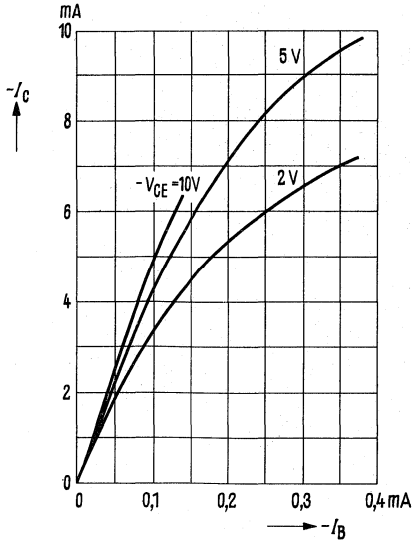
Collector current I_C = f(V_B) V_{CE} = \text{parameter} (common emitter configuration)
