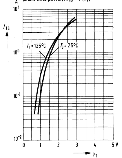
Forward characteristic (short-time power); I_{TS} = f(V_T)
