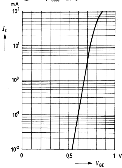
Collector current I_C = f(V_{BE}) V_{CE} = 10 \text{ V}; T_{case} = 25 \text{ }^\circ\text{C}
