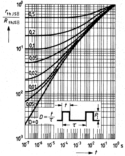
Perm. pulse load \frac{r_{thJSB}}{R_{thJSB}} = f(t) D = \text{parameter}
