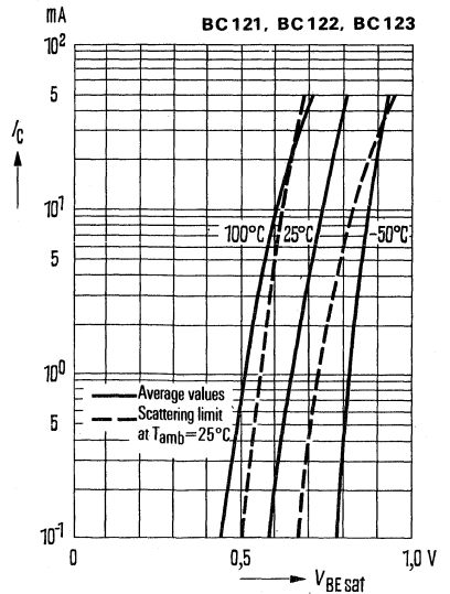
Base-emitter saturation voltage V_{BE\text{sat}} = f(I_C) h_{FE} = 20 ; T_{\text{amb}} = \text{parameter} (common emitter configuration)
