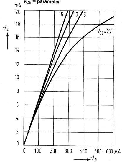
Collector current I_C = f(I_B) V_{CE} = \text{parameter}
