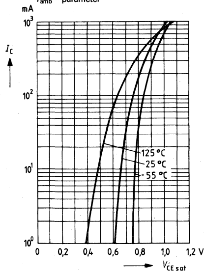
Collector emitter saturation voltage V_{CEsat} = f(I_C); h_{FE} = 1000 T_{amb} = \text{parameter}
