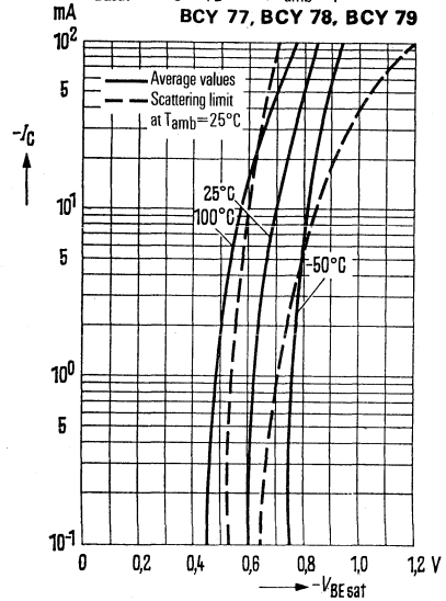
Base-emitter saturation voltage V_{BEsat} = f(I_C); h_{FE} = 40; T_{amb} = \text{parameter}
