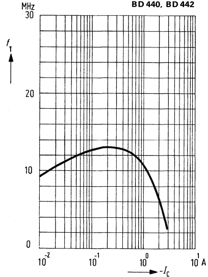
Transition frequency f_T = f(I_C) T_{\text{case}} = 25^\circ\text{C}
