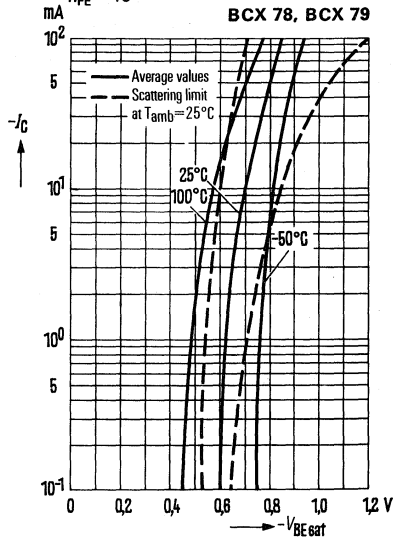
Base-emitter saturation voltage V_{BEsat} = f(I_C); T_{\text{amb}} = \text{parameter}; h_{FE} = 40
