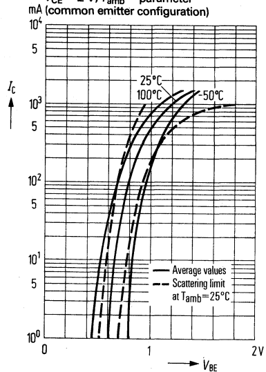
Collector current I_C = f(V_{BE}) V_{CE} = 2\text{ V}; T_{amb} = \text{parameter} (common emitter configuration)
