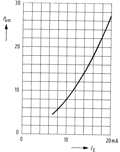
Oscillator output power
