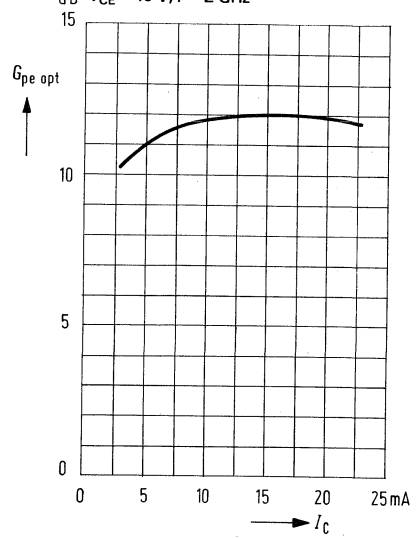
Max. power gain
