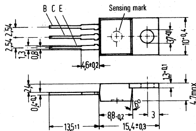
Approx. weight 18 g Dimensions in mm
