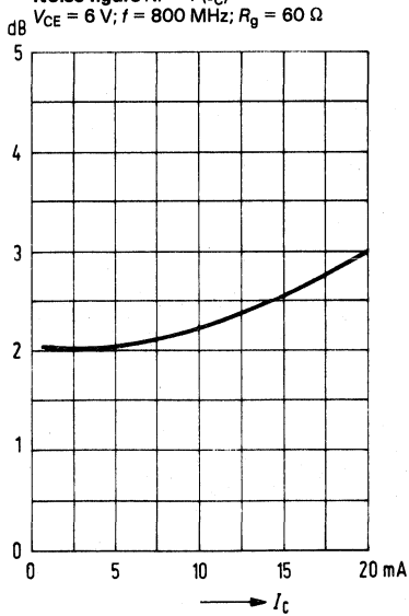
Noise figure NF = f(I_C)
