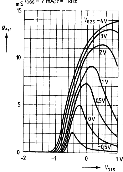
Gate 1 transadmittance g_{fs1} = f(V_{G1S}) :
