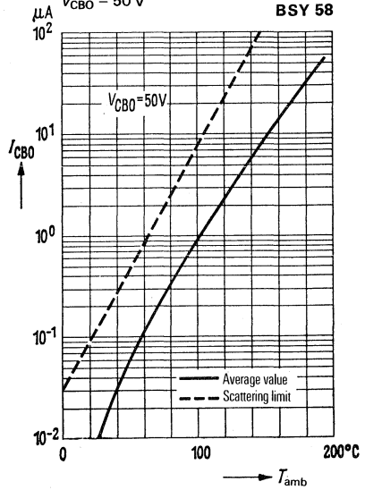
Collector cutoff current versus temperature I_{CBO} = f(T_{amb}) V_{CBO} = 50\text{ V}
