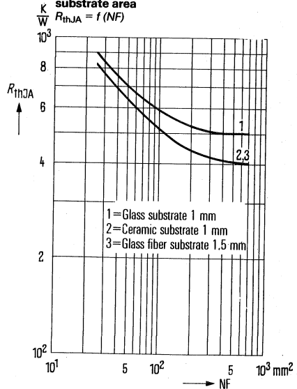
Thermal resistance versus substrate area
