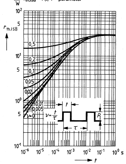
Permissible pulse load r_{th,JSB} = f(t) \quad v = \text{parameter}
