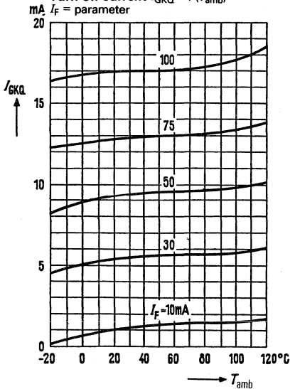
Turn-off current I_{GKQ} = f(T_{amb}) I_F = \text{parameter}
