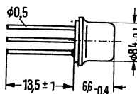
Approx. weight 1.5 g
