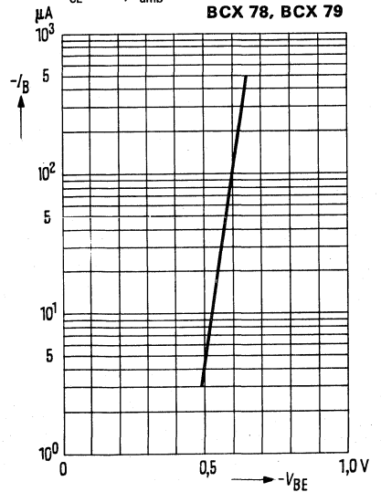
Input characteristic I_B = f(V_{BE}) V_{CE} = 5V; T_{amb} = 25^\circ C
