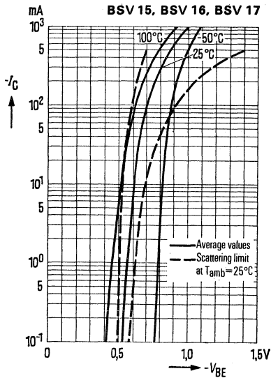
Collector current I_C = f(V_{BE}) -V_{CE} = 1V; T_{amb} = \text{parameter}
