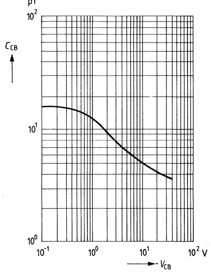
Collector-base capacitance C_{CB} = f(V_{CB}); T_{amb} = 25^{\circ}C
