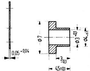
Insulating nipple
