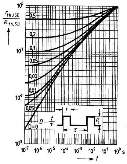
Pulse resistance r_{thJSB} = f(t) D = \text{parameter} \frac{r_{thJSB}}{R_{thJSB}} = f(t)
