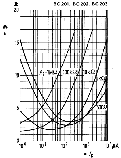
Noise figure NF = f(I_C) -V_{CE} = 5V; f = 1\text{ kHz}; T_{amb} = 25^\circ C
