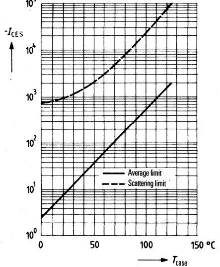
Collector cutoff current versus temperature I_{CES} = f(T_{\text{case}})
