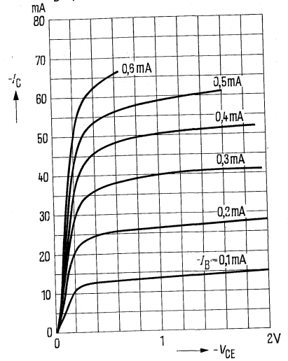
Output characteristics I_C = f(V_{CE}) I_B = \text{parameter}
