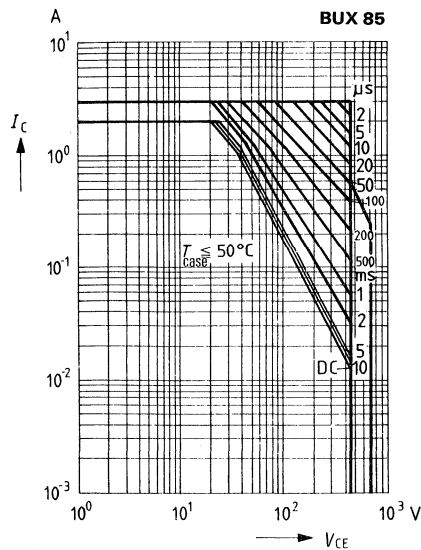
Permissible operating range
