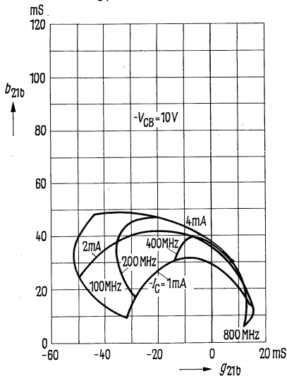
Small signal short circuit forward transfer admittance y_{21b} ; -V_{CB} = 10\text{ V} (common base configuration) measuring plane 5 mm below case bottom
