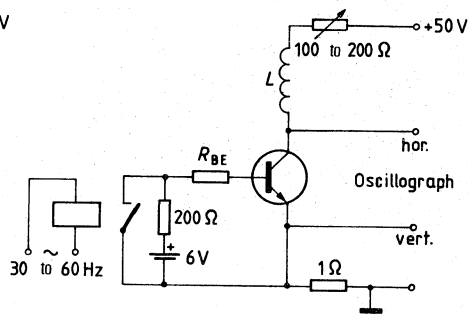
for V_{(BR)CER}
