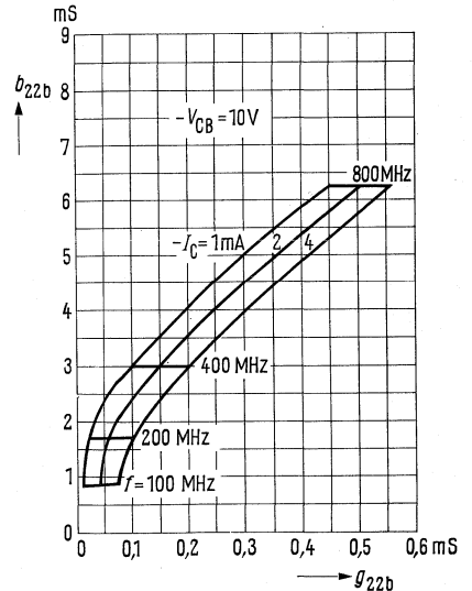
Small signal short circuit output admittance y_{22b} ; -V_{CB} = 10\text{ V} (common base configuration) measuring plane 5 mm below case bottom
