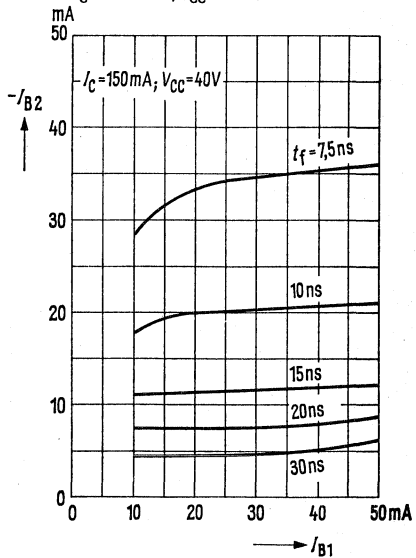
Fall time t_f I_C = 150 \text{ mA}; V_{CC} = 40 \text{ V}
