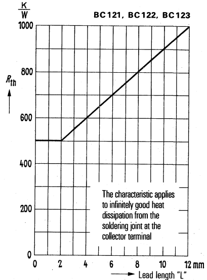
Thermal resistance R_{th} = f(\text{lead length "L"})
