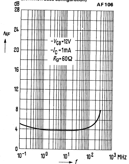
Noise figure versus frequency NF = f(f) ; -V_{CB} = 12V ; -I_C = 1mA ; R_g = 60 \Omega (common base configuration)
