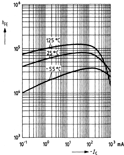
DC current gain h_{FE} = f(I_C) -V_{CE} = 2\text{ V}; T = \text{parameter}
