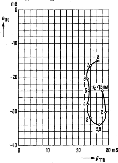
Small signal short circuit input transfer admittance y_{11b} (common base configuration) -V_{CC} = 12\text{ V}; R_{EE} = 1\text{ k}\Omega; f = 200\text{ MHz}
