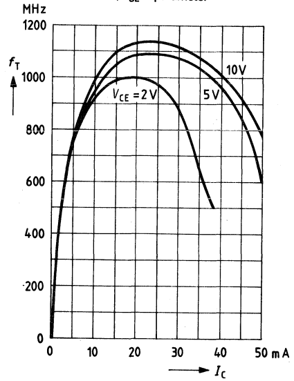
Transition frequency f_T = f(I_C) f = 100 MHz; V_{CE} = \text{parameter}
