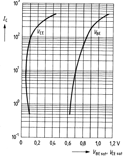
Saturation voltages
