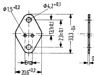
Mica washer dry: R_{th} = 2.5 \text{ K/W} greased: R_{th} = 1 \text{ K/W}
