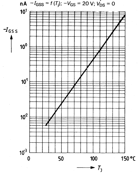
Reverse current versus temperature
