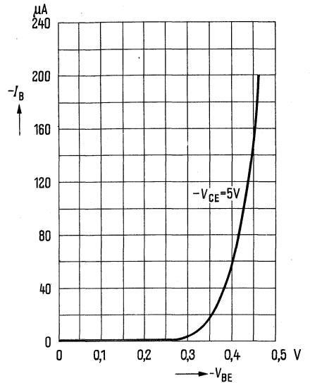
Input characteristic I_B = f(V_{BE}) -V_{CE} = 5 V (common emitter configuration)
