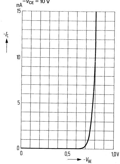
Input characteristic I_C = f(V_{BE}) -V_{CE} = 10\text{ V}
