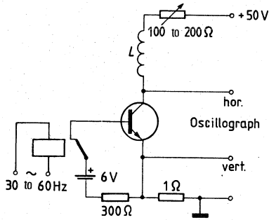
for V_{(BR)CE0}
