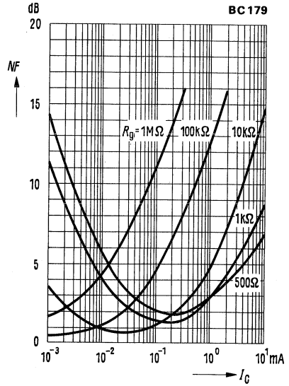
Noise figure NF = f(I_C) -V_{CE} = 5\text{ V}; f = 1\text{ kHz}; T_{amb} = 25^\circ\text{C}
