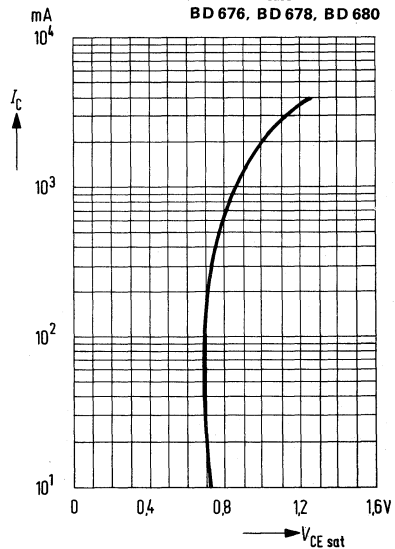
Collector-emitter saturation voltage V_{CE\text{sat}} = f(I_C); h_{FE} = 100; T_{\text{case}} = 25^\circ\text{C}
