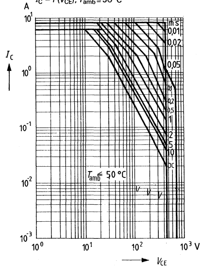
Permissible operating range I_C = f(V_{CE}); T_{amb} \leq 50^{\circ}C
