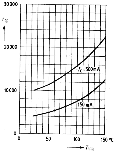
DC current gain h_{FE} = f(T_{amb}) -I_C = parameter; -V_{CE} = 10 \text{ V}
