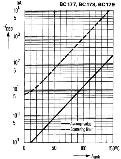
Collector cutoff current versus temperature I_{CBO} = f(T_{\text{amb}}) (for max. permissible reverse voltage)
