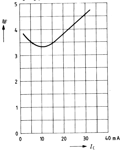
Noise figure NF = f(I_C) dB Z_g = Z_{g,opt}; V_{CE} = 10\text{ V}; f = 2\text{ GHz}
