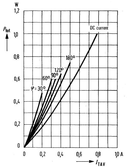
Power dissipation (sine) P_{tot} = f(I_{TAV}) f = 50 \text{ to } 400 \text{ Hz}; T = 125^\circ\text{C}
