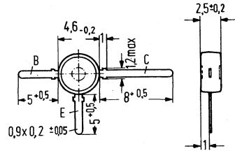
Approx. weight 0.3 g Dimensions in mm
