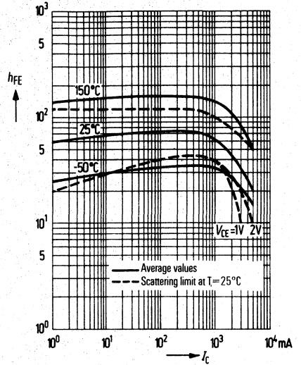
DC current gain h_{FE} = f(I_C) T_{case} = \text{parameter}
