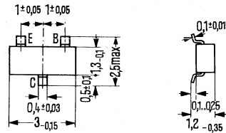
Approx. weight 0.02 g Dimensions in mm
