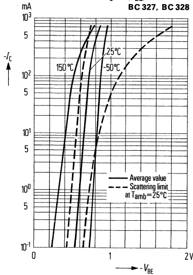
Collector current I_C = f(V_{BE}) BC 327, BC 328
