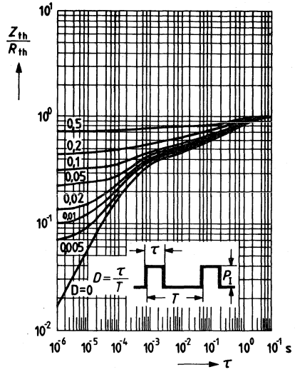
Permissible pulse load r_{thJA} = f(t)
