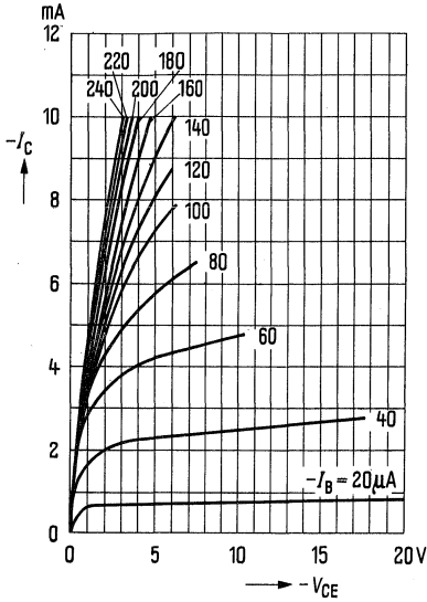
Output characteristics I_C = f(V_{CE}) ; (common emitter configuration)
