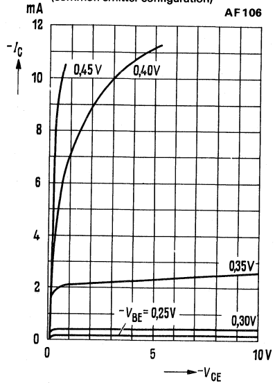
Output characteristics I_C = f(V_{CE}) ; V_{BE} = parameter (common emitter configuration)
