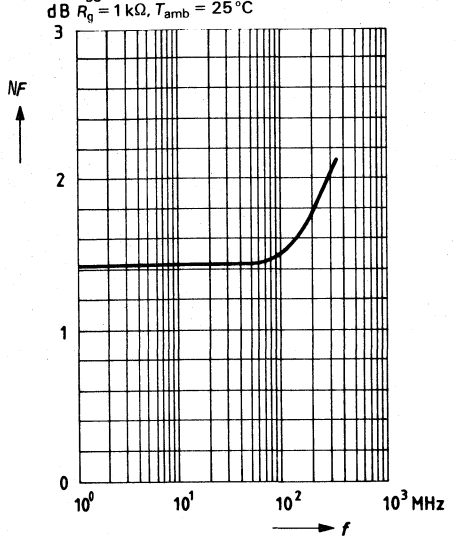
Noise figure NF = f(f)
