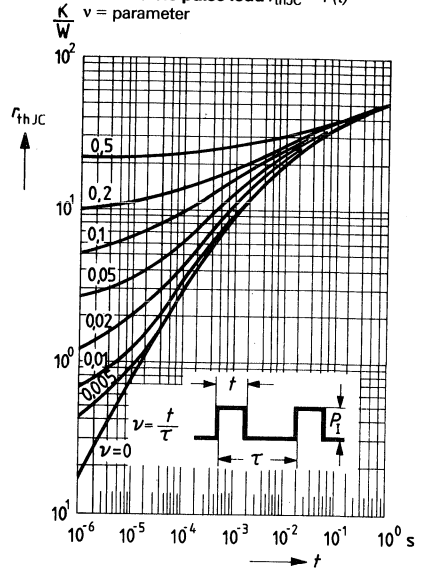
Permissible pulse load r_{thJC} = f(t)
