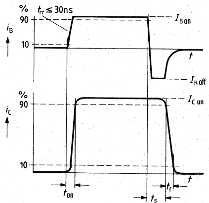
Timing diagram
