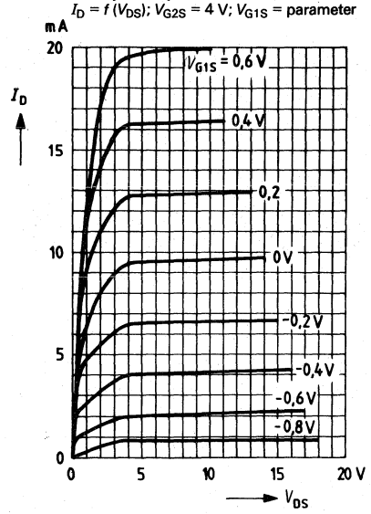
Family of output characteristics
