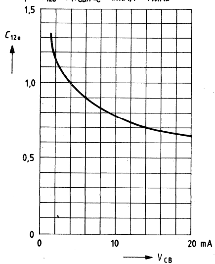
Reverse transfer capacitance C_{12e} = f(V_{CB}) ; I_C = 1 mA; f = 1 MHz
