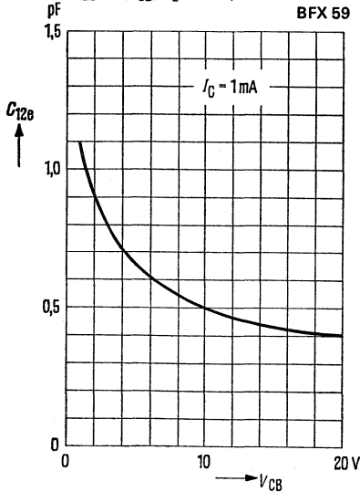
Reverse transfer capacitance C_{12e} = f(V_{CB}) ; I_C = 1 \text{ mA} ; f = 1 \text{ MHz}
