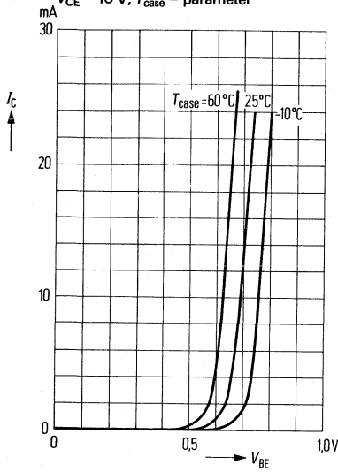
Collector current I_C = f(V_{BE}) V_{CE} = 10\text{ V}; T_{\text{case}} = \text{parameter}
