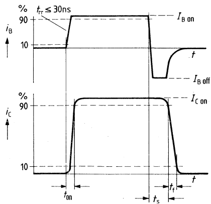
Timing diagram
