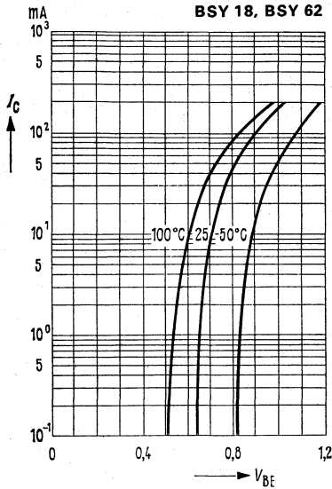
Collector current I_C = f(V_{BE}) V_{CE} = 1\text{ V} (common emitter configuration)
