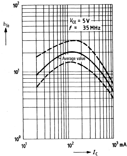
Small signal current gain h_{fe} = f(I_C)
