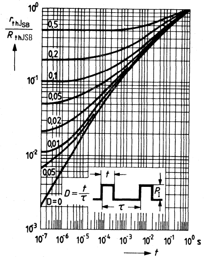
Perm. pulse load r_{thJSB} = f(t) D = \text{parameter}
