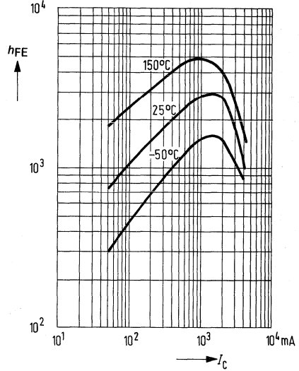
DC current gain h_{FE} = f(I_C) -V_{CE} = 3 \text{ V}
