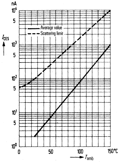
Collector-cutoff current versus temperature I_{CES} = f(T_{amb})
