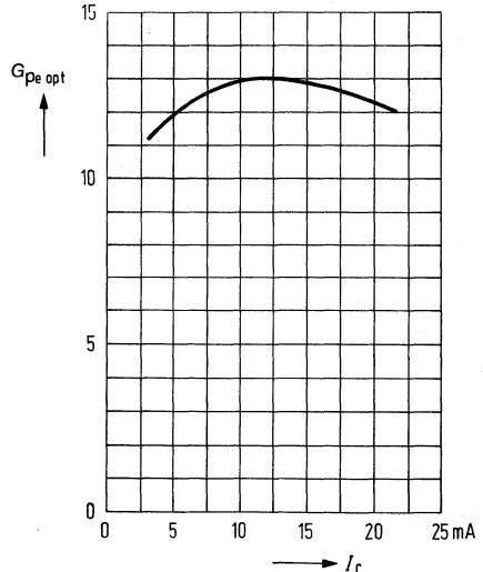
Max. pp power gain G_{pe\ opt} = f(I_C)
