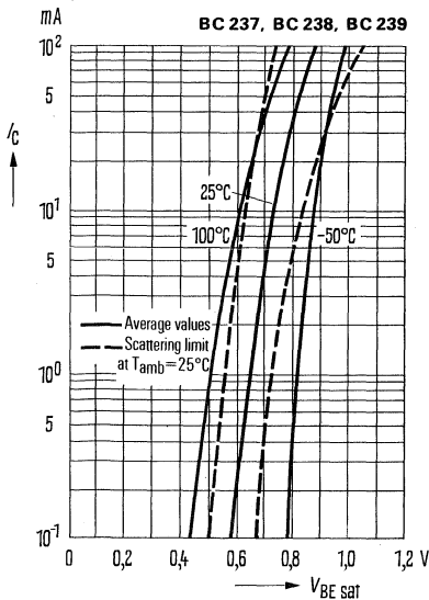
Base-emitter saturation voltage V_{BEsat} = f(I_C); T_{amb} = \text{parameter}; h_{FE} = 20 (common emitter configuration)
