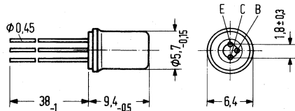
Approx. weight 1 g
