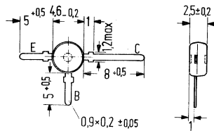
Approx. weight 0.25 g Dimensions in mm
