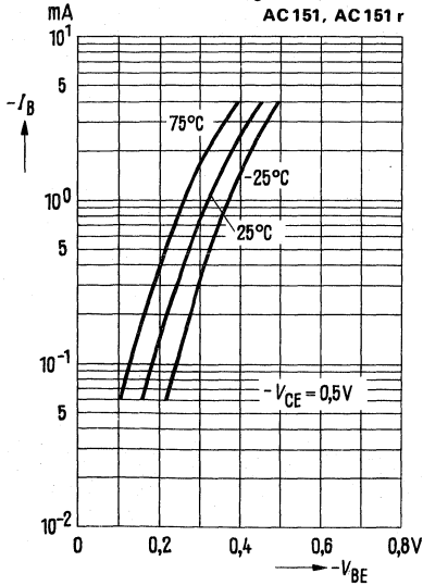
Input characteristics I_B = f(V_{BE}) -V_{CE} = 0.5 \text{ V}; T_{amb} = \text{parameter} (common emitter configuration)
