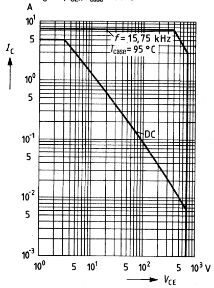
Permissible operating range I_C = f(V_{CE}); T_{case} = 95^{\circ}C
