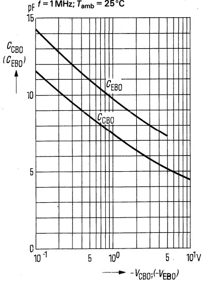
Emitter-base capacitance C_{EBO} = f(V_{EBO})
