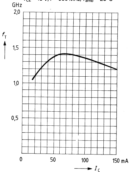
Transition frequency f_T = f(I_C) V_{CE} = 15 \text{ V}, f = 500 \text{ MHz}, T_{amb} = 25 \text{ °C}
