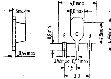
Approx. weight 0.1 g Dimensions in mm
