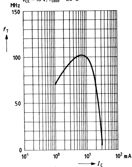
Transition frequency f_T = f(I_C) V_{CE} = 10 \text{ V}; T_{\text{case}} = 25^\circ\text{C}
