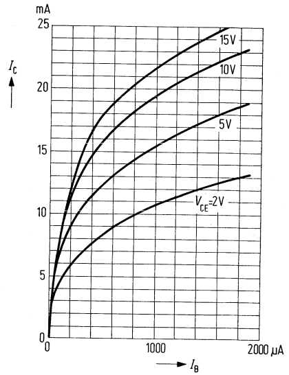
Collector current I_C = f(I_B)
