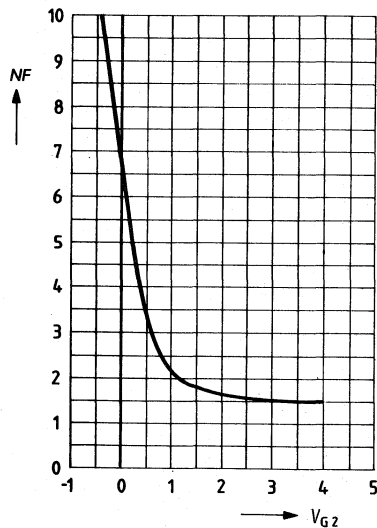
Noise figure NF = f(V_{G2S}) V_{DS} = 15\text{ V} ; V_{G1S} = 0 I_{DSS} = 10\text{ mA} ; f = 200\text{ MHz} R_S = 0\Omega (see figure 1)
