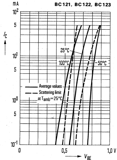
Collector current I_C = f(V_{BE}) T_{amb} = parameter; V_{CE} = 2 V (common emitter configuration)
