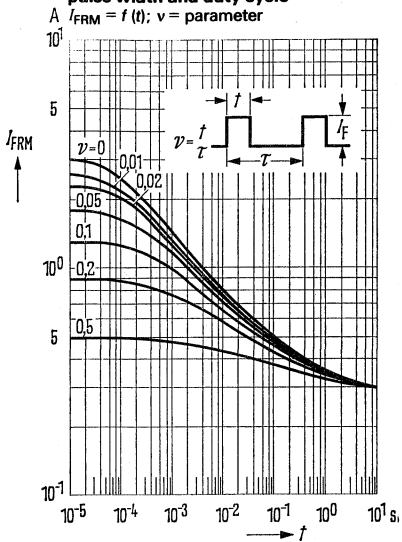
Permissible anode current versus pulse width and duty cycle I_{FRM} = f(t); v = \text{parameter}
