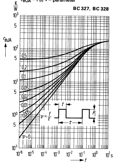
Permissible pulse load r_{thJA} = f(t) \nu = \text{parameter}
