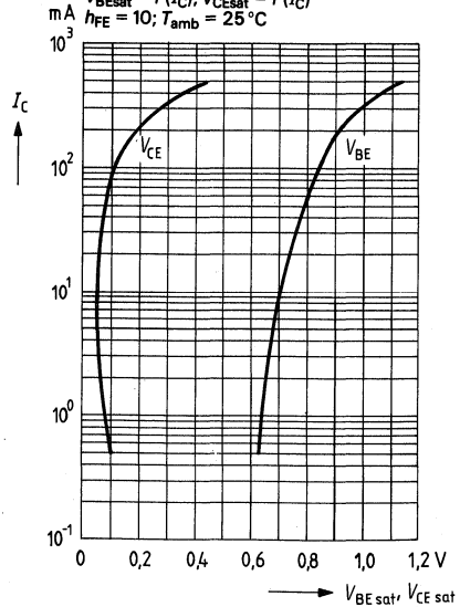
Saturation voltages
