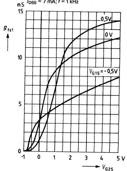
Gate 2 transadmittance g_{fs1} = f(V_{G2S}) :
