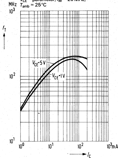
Transition frequency f_T = f(I_C) V_{CE} = \text{parameter}; f_M = 20 \text{ MHz}; T_{amb} = 25^\circ\text{C}
