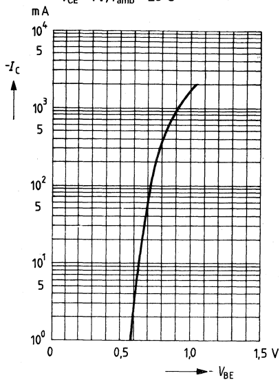
Collector current I_C = f(V_{BE}) -V_{CE} = 1\text{ V}; T_{amb} = 25^\circ\text{C}
