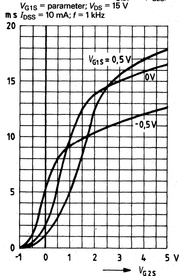
Gate 2 transmittance g_{fs2} = f(V_{G2S})
