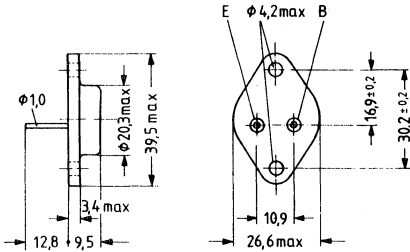
Approx. weight 18 g Dimensions in mm
