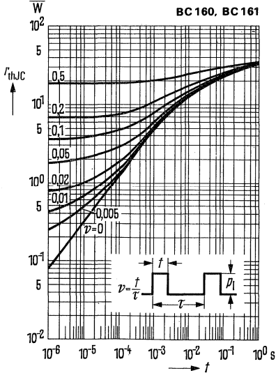
Permissible pulse load i_{thJC} = f(t); v = \text{parameter}
