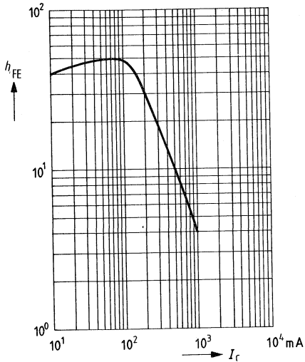
DC current gain h_{FE} = f(I_C) V_{CE} = 5 \text{ V}; T_{amb} = 25^\circ\text{C}
