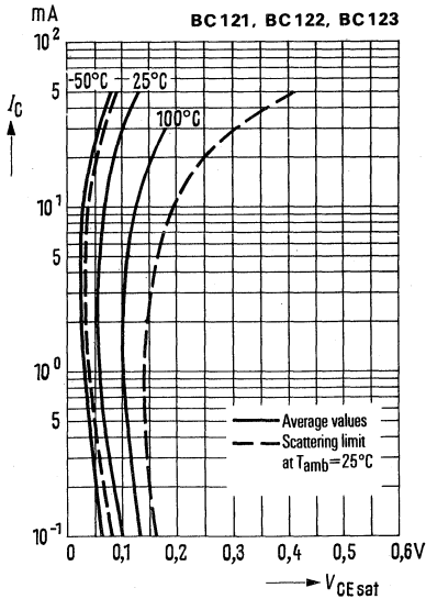
Collector-emitter saturation voltage V_{CE\text{sat}} = f(I_C) h_{FE} = 20 ; T_{\text{amb}} = \text{parameter} (common emitter configuration)
