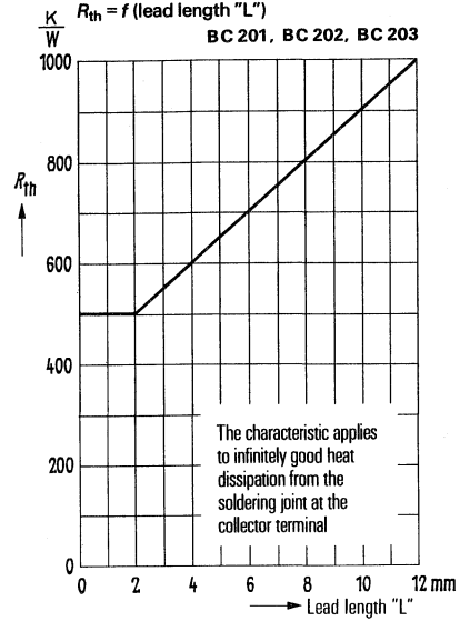
Thermal resistance R_{th} = f(\text{lead length "L"})
