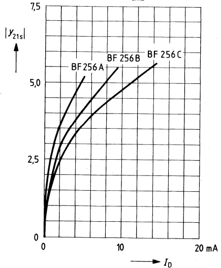
Small-signal short-circuit forward transfer admittance
