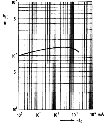
DC current gain h_{FE} = f(I_C) -V_{CE} = 1 V, T_{amb} = 25^\circ C
