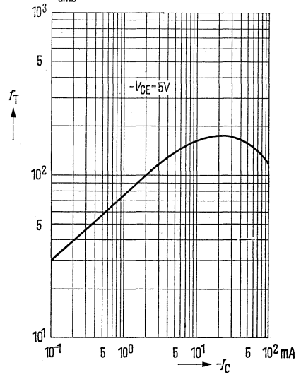
Transition frequency f_T = f(I_C) MHz T_{amb} = 25^\circ\text{C}
