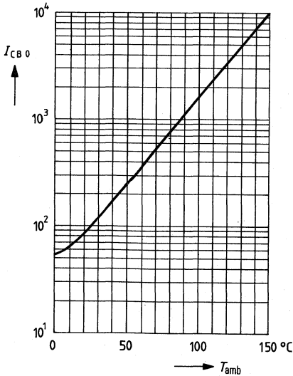
Collector cutoff current versus temperature I_{CB0} = f(T_{amb}) V_{CB} = V_{CBmax}
