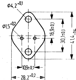
Mica washer dry: R_{th} = 1.25 \text{ K/W} greased: R_{th} = 0.35 \text{ K/W}
