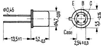
Approx. weight 0.4 g Dimensions in mm
