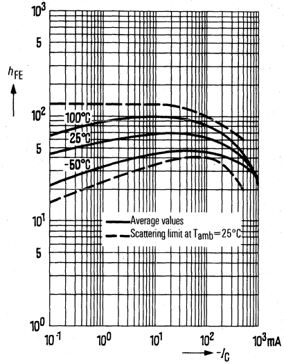
DC current gain h_{FE} = f(I_C) -V_{CE} = 1 \text{ V} ; T_{amb} = \text{parameter} BSV 15-6, BSV 16-6, BSV 17-6
