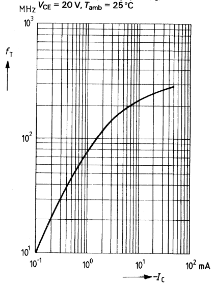
Transition frequency f_T = f(I_C) V_{CE} = 20 V, T_{amb} = 25^\circ C
