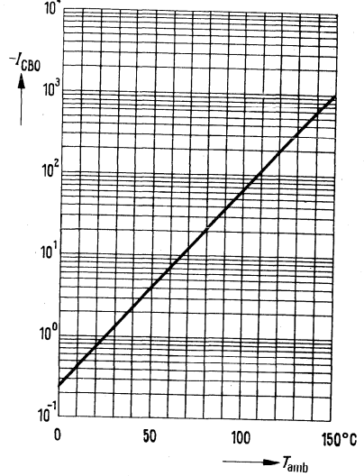
Collector cutoff current versus temperature I_{CBO} = f(T_{amb}) I_A - V_{CB} = 60 \text{ V}
