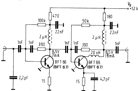
Circuit 2
