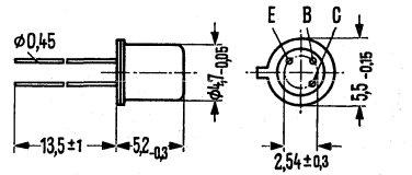
Approx. weight 0.3 g
