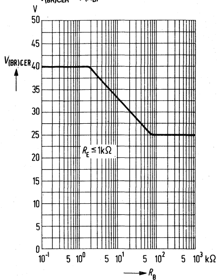
Min.-limit characteristic of collector-emitter breakdown voltage
