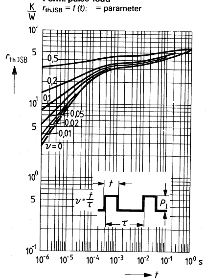
Perm. pulse load r_{thJSB} = f(t); = \text{parameter}
