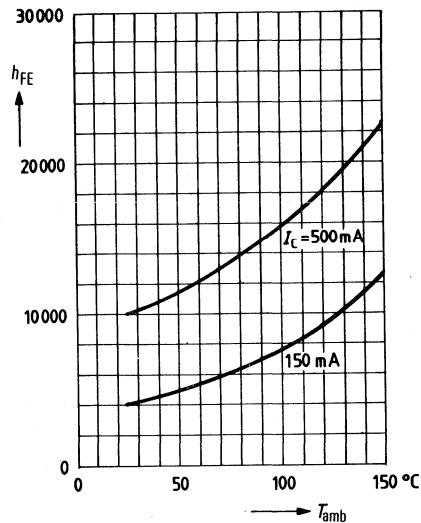
DC current gain h_{FE} = f(T_{amb})
