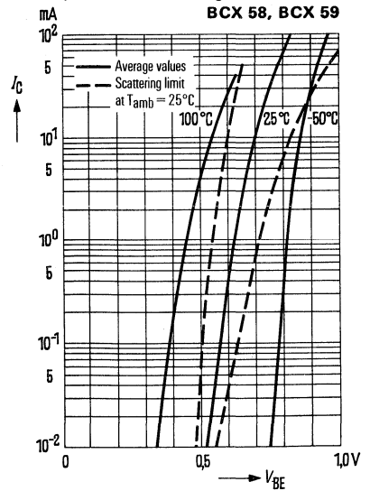
Collector current I_C = f(V_{BE}) V_{CE} = 1\text{V} (common emitter configuration)
