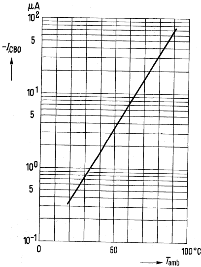
Collector cutoff current I_{CBO} = f(T_{\text{amb}}) ; versus temperature -V_{CB0} = 20 \text{ V}
