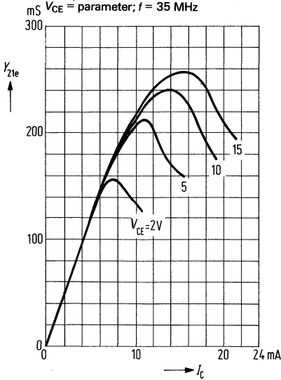
Small-signal short-circuit forward transfer admittance |y_{21e}| = f(I_C) V_{CE} = \text{parameter}; f = 35\text{ MHz}
