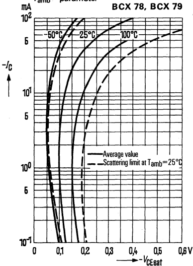
Collector-emitter saturation voltage V_{CEsat} = f(I_C); h_{FE} = 40; T_{\text{amb}} = \text{parameter}
