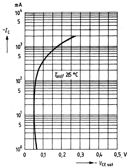
Collector-emitter saturation voltage V_{CEsat} = f(I_C) h_{FE} = 10; T_{amb} = 25^\circ\text{C}
