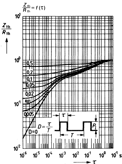
Total perm. power dissipation
