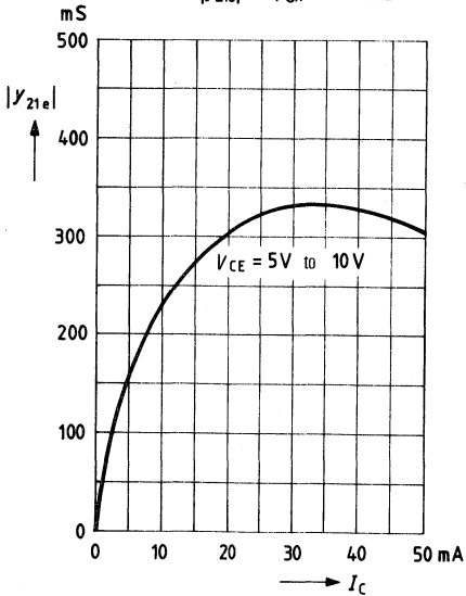
Short-circuit forward transfer admittance |y_{21e}| = f(I_C) , f = 35 MHz
