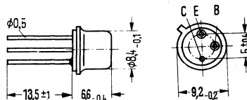
Approx. weight 1.5 g Dimensions in mm
