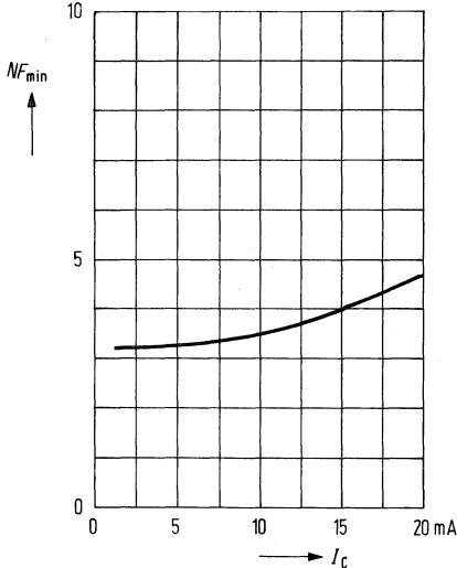
Min. noise figure NF_{min} = f(I_C)
