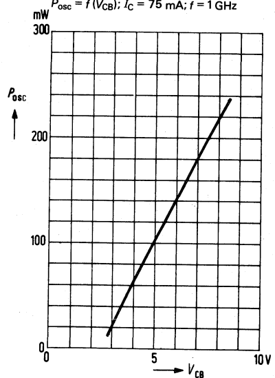
Oscillator output power P_{osc} = f(V_{CB}); I_C = 75\text{ mA}; f = 1\text{ GHz}
