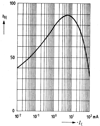
DC current h_{FE} = f(I_C) V_{CE} = 5 V; T_{amb} = 25^{\circ}C
