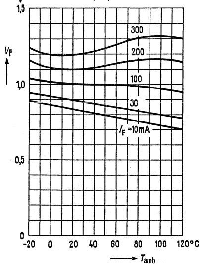
Forward voltage V_F = f(T_{amb}) Forward current I_F = \text{parameter}
