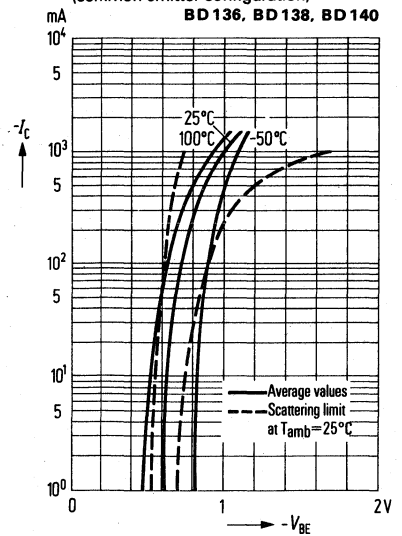
Collector current I_C = f(V_{BE}) V_{CE} = 2\text{ V}; T_{amb} = \text{parameter} (common emitter configuration) BD 136, BD 138, BD 140
