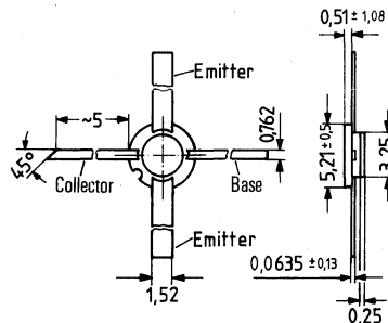
Approx. weight 0.08 g Dimensions in mm
