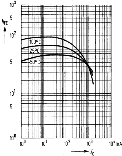
DC current gain h_{FE} = f(I_C) V_{CE} = 2\text{ V}; T_{amb} = \text{parameter}
