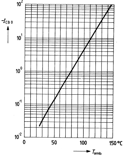
Collector cutoff current versus temperature I_{CBO} = f(T_{amb}) V_{CB} = 100 V
