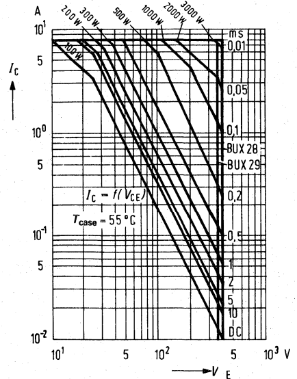
Permissible operating range I_C = f(V_{CE}); T_{case} = 55^\circ C; v = 0
