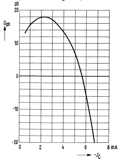
Power gain G_{pb} = f(I_C) ; f = 500 \text{ MHz}; -V_{batt} = 10 \text{ V}; R_V = 1 \text{ k}\Omega; R_L = 2 \text{ k}\Omega (common base configuration)
