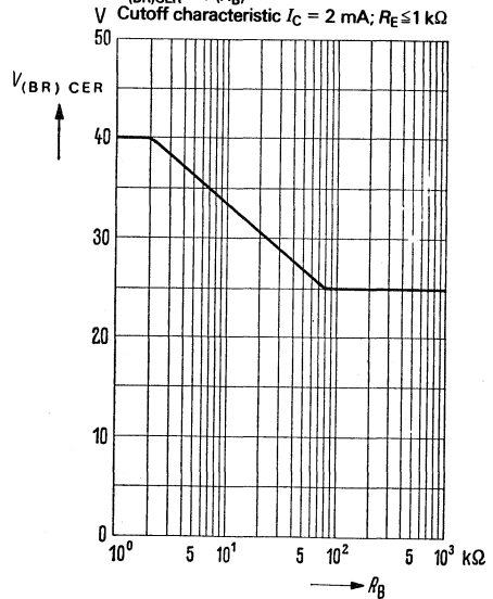
Collector-emitter breakdown voltage V_{(BR)CER} = f(R_B) Cutoff characteristic I_C = 2\text{ mA} ; R_E \leq 1\text{ k}\Omega
