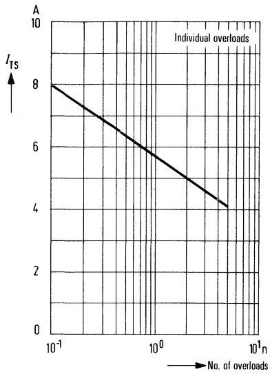
Surge on-state current I_{TS} = f(\text{overloads at 50 Hz})
