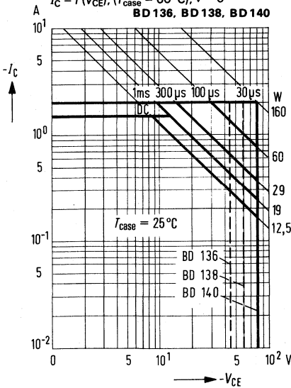
Permissible operating range I_C = f(V_{CE}); (T_{case} = 60^\circ\text{C}); v = 0 BD 136, BD 138, BD 140
