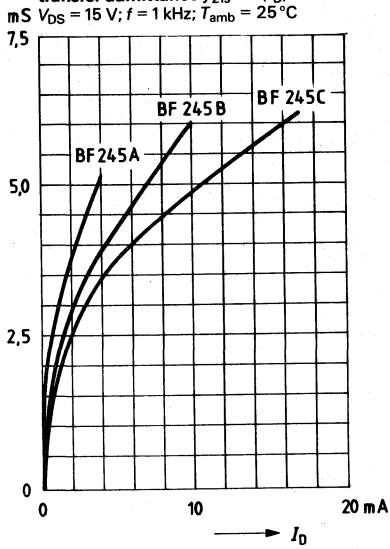
Small-signal short-circuit forward transfer admittance y_{21s} = f(I_D)
