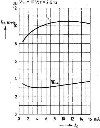
Gain at noise matching
