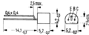
Mounting instruction: Fixing hole dia 0.6 Approx. weight 0.25 g Dimensions in mm
