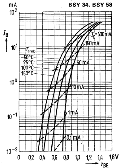
Input characteristics I_B = f(V_{BE}) V_{CE} = 1\text{ V} (common emitter configuration)
