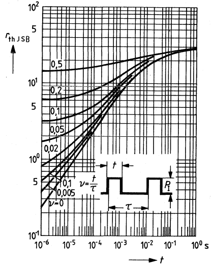
Permissible pulse load r_{thJSB} = f(t) \text{ v = parameter}
