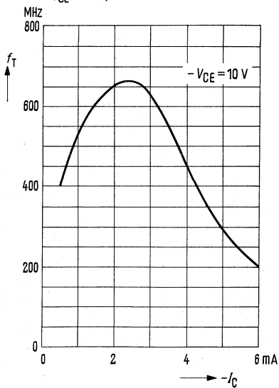
Transition frequency f_T = f(I_C) ; -V_{CE} = 10 \text{ V}; f = 100 \text{ MHz}
