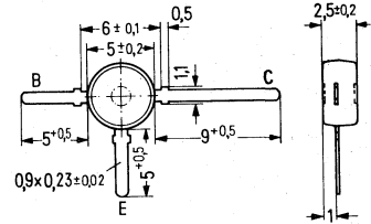
Approx. weight 0.3 g Dimensions in mm
