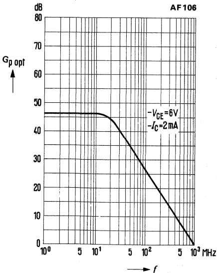
Optimum power gain G_{p,opt} = f(f) -V_{CE} = 6V ; -I_C = 2mA (common emitter configuration)
