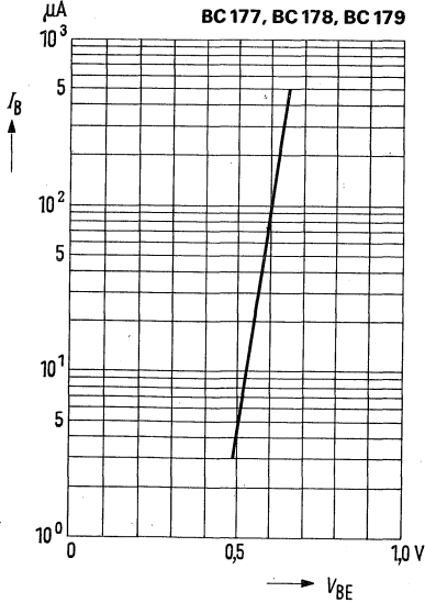
Input characteristic: I_B = f(V_{BE}) -V_{CE} = 5\text{ V}; T_{\text{amb}} = 25^\circ\text{C}
