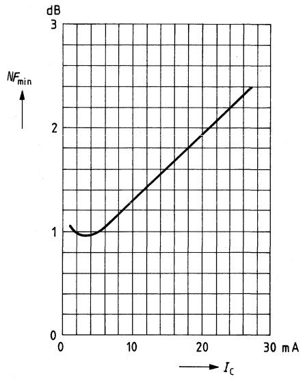
Noise figure NF_{min} = f(I_C) V_{CE} = 6\text{ V}; R_{g,opt}; f = 10\text{ MHz}
