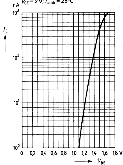
Collector current I_C = f(V_{BE}) V_{CE} = 2 V; T_{amb} = 25^{\circ}C
