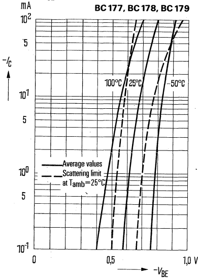
Collector current I_C = f(V_{BE}) -V_{CE} = 5\text{ V}
