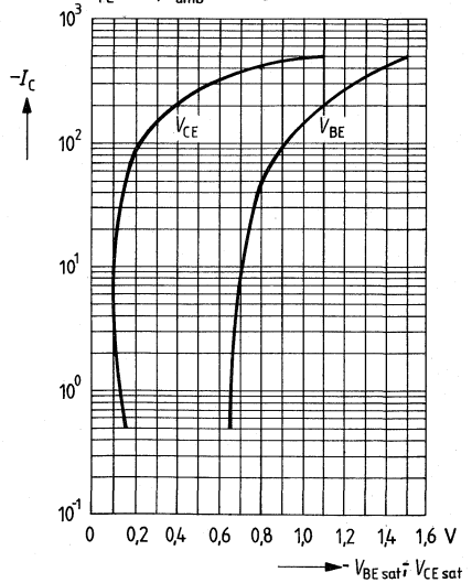
Saturation voltages V_{BEsat} = f(I_C), V_{CEsat} = f(I_C) h_{FE} = 10; T_{amb} = 25^{\circ}C
