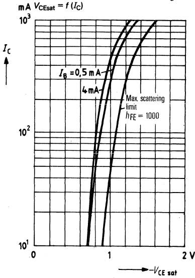
Collector-emitter saturation voltage
