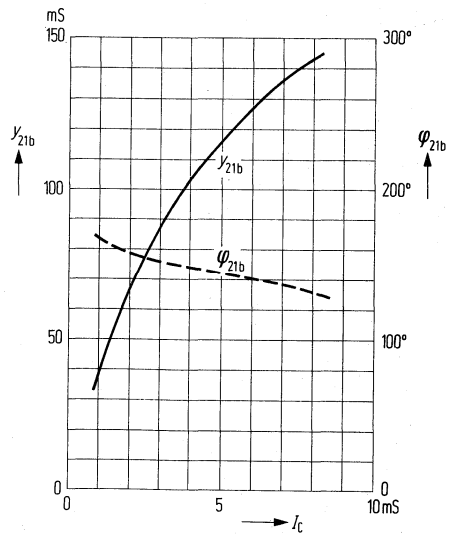
Short-circuit forward transfer admittance
