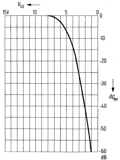
Power gain control range
