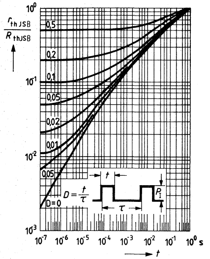
Pulse resistance \frac{r_{thJSB}}{R_{thJSB}} = f(t) D = parameter
