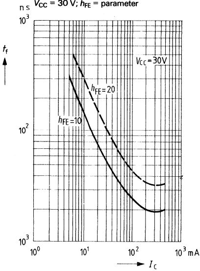
Fall time t_f = f(I_C) V_{CC} = 30 V; h_{FE} = \text{parameter}
