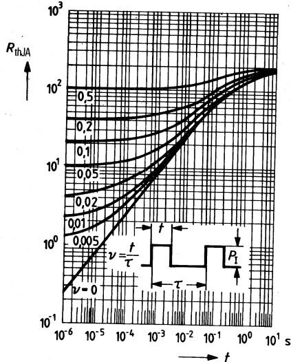
Permissible pulse load
