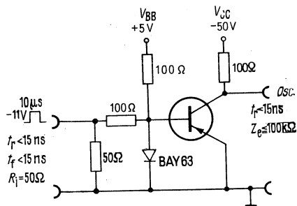
Test circuit for switching times
