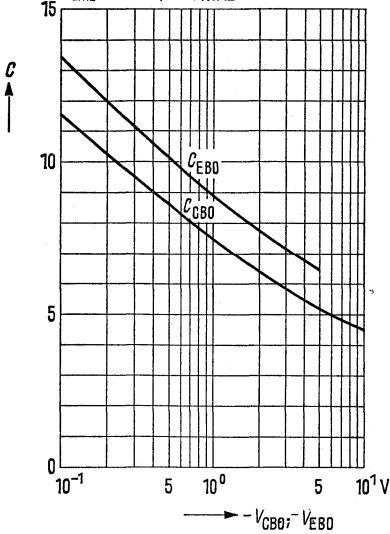
Emitter-base capacitance
