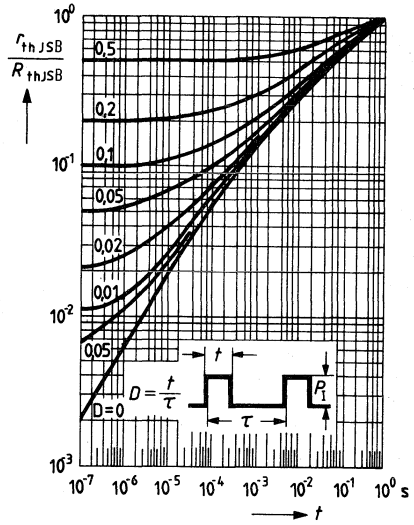
Pulse resistance \frac{r_{thJSB}}{R_{thJSB}} = f(t) D = \text{parameter}
