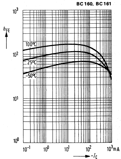
DC current gain h_{FE} = f(I_C) -V_{CE} = 1V; T_{amb} = \text{parameter} (common emitter configuration)
