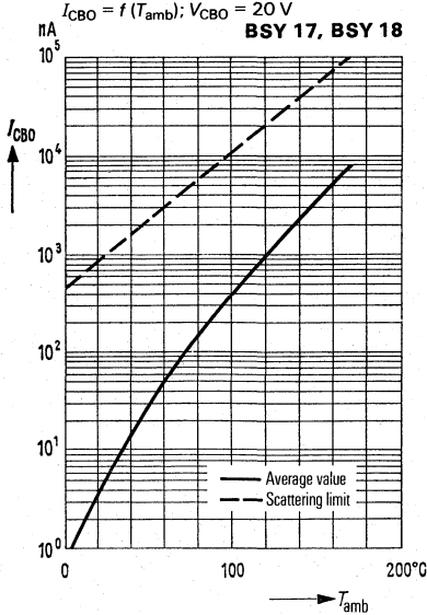
Collector cutoff current versus temperature I_{CBO} = f(T_{\text{amb}}); V_{CBO} = 20\text{ V}
