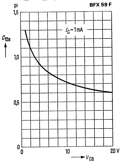
Reverse transfer capacitance C_{12e} = f(V_{CB}); I_E = 1 \text{ mA}; f = 1 \text{ MHz}
