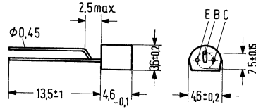
Approx. weight 0.25 g Dimensions in mm
