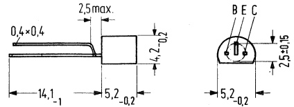
Approx. weight 0.25 g Dimensions in mm
