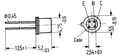
Approx. weight 0.4 g
