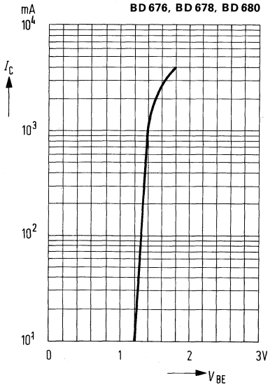
Collector current I_C = f(V_{BE}) -V_{CE} = 3 \text{ V}; T_{\text{case}} = 25^\circ\text{C}
