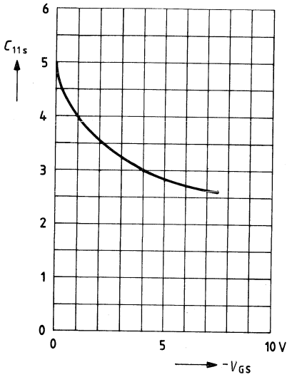
Input characteristics C_{11S} = f(-V_{GS})
