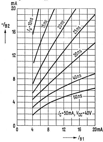
Storage time t_s I_C = 50 \text{ mA}; V_{CC} = 40 \text{ V}
