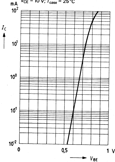
Collector current I_C = f(V_{BE}) V_{CE} = 10 \text{ V}; T_{case} = 25^\circ\text{C}
