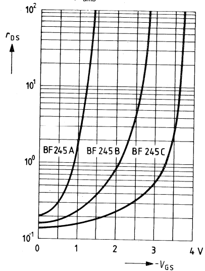
Dynamic drain-source resistance
