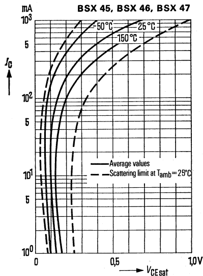
Saturation voltage V_{CEsat} = f(I_C) h_{FE} = 10; T_{amb} = \text{parameter}
