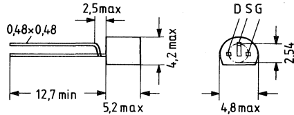
Approx. weight 0.25 g Dimensions in mm
