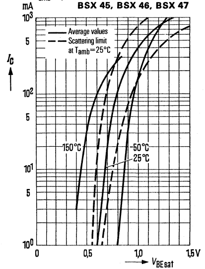
Saturation voltage V_{BEsat} = f(I_C) h_{FE} = 10; V_{CE} = 1 \text{ V}; T_{amb} = \text{parameter}
