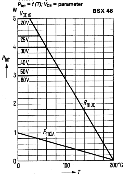
Total perm. power dissipation versus temperature
