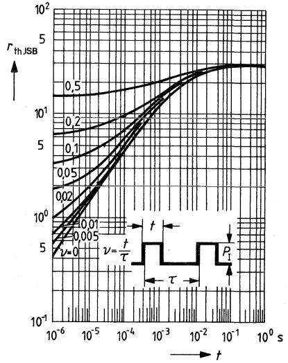
Permissible pulse load r_{thJSB} = f(t) \nu = \text{parameter}
