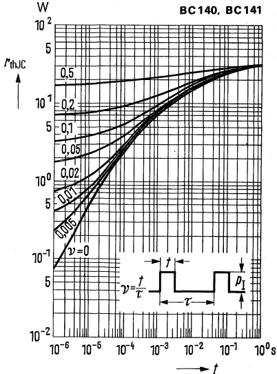
Permissible pulse load r_{thJC} = f(f); v = \text{parameter}
