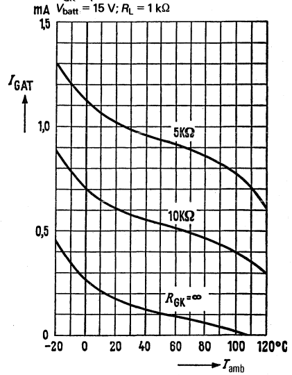
Anode control current I_{GAT} = f(T_{amb}) R_{GK} = \text{parameter} V_{batt} = 15\text{ V}; R_L = 1\text{ k}\Omega
