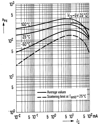
DC current gain h_{FE} = f(I_C) V_{CE} = 1\text{V}; T_{amb} = \text{parameter} (common emitter configuration) BCX 58 VIII, BCX 59 VIII
