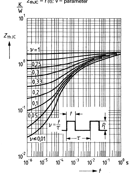
Permissible pulse load Z_{thJC} = f(t); v = \text{parameter}
