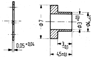
Insulating nipple scale 2:1
