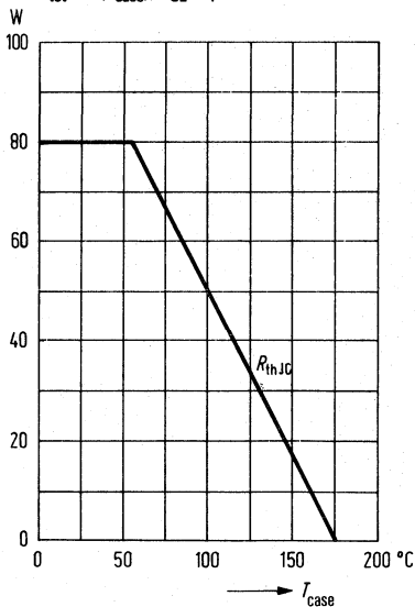
Total perm. power dissipation versus temperature P_{tot} = f(T_{case}); V_{CE} = \text{parameter}
