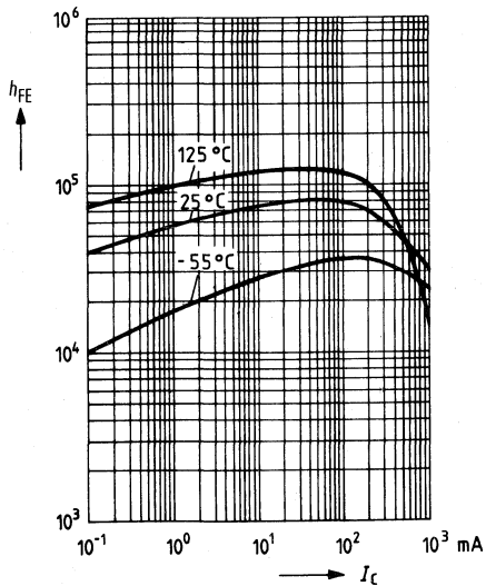
DC current gain h_{FE} = f(I_C) : V_{CE} = 2 V; T_{amb} = \text{parameter}
