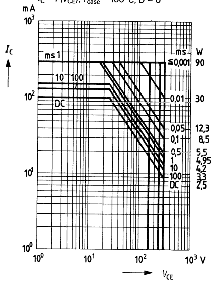
Permissible operating range I_C = f(V_{CE}); T_{case} = 100^\circ\text{C}; D = 0
