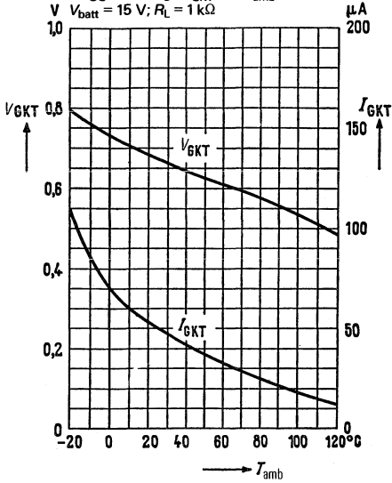
Trigger current I_{GKT} = f(T_{amb}) Trigger voltage V_{GKT} = f(T_{amb}) V_{batt} = 15\text{ V}; R_L = 1\text{ k}\Omega
