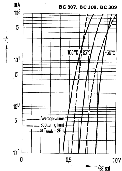
Base-emitter saturation voltage V_{BEsat} = f(I_C); h_{FE} = 20; T_{amb} = \text{parameter}
