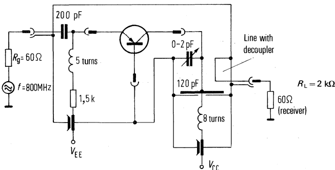
Test circuit for power gain and noise figure at f = 800\text{ MHz}
