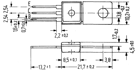
Approx. weight 15 g. Dimensions in mm
