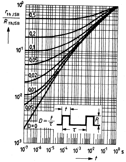
Pulse resistance \frac{r_{\text{thJSB}}}{R_{\text{thJSB}}} = f(t) D = parameter
