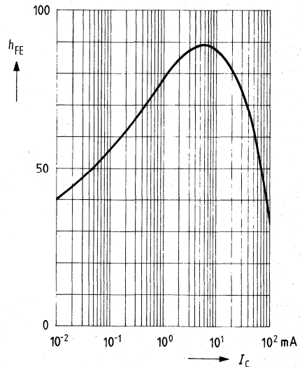
DC current gain h_{FE} = f(I_C) V_{CE} = 5 V; T_{amb} = 25^{\circ}C
