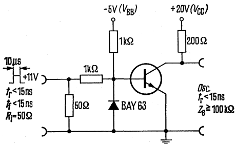
Test circuit for switching times
