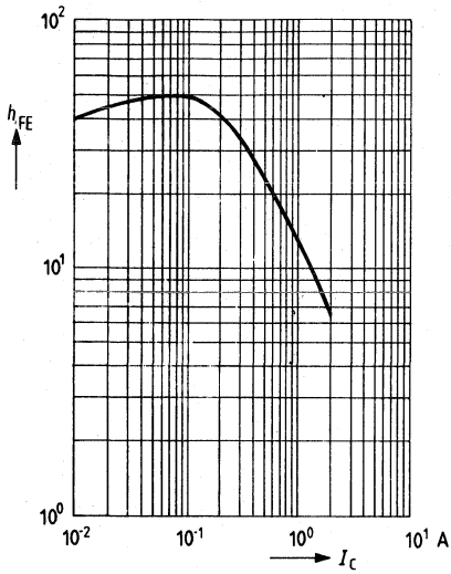
DC current gain h_{FE} = f(I_C) V_{CE} = 5 \text{ V}; T_{\text{case}} = 25^\circ\text{C}
