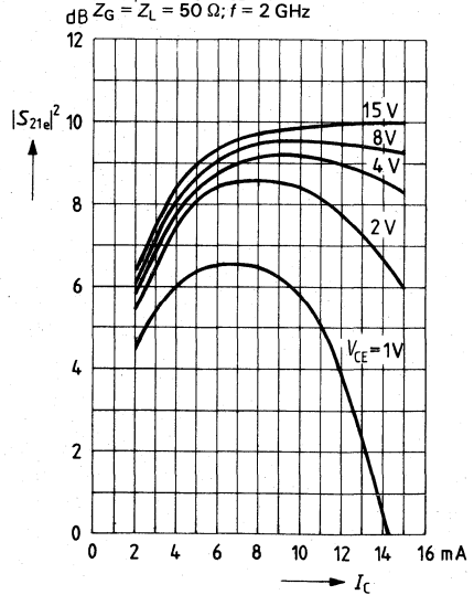
Insertion gain
