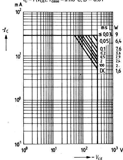
Permissible operating range I_C = f(V_{CE}); T_{case} = \leq 110^\circ\text{C}; D = 0.01
