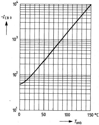
Collector cutoff current versus temperature I_{CB0} = f(T_{amb})
