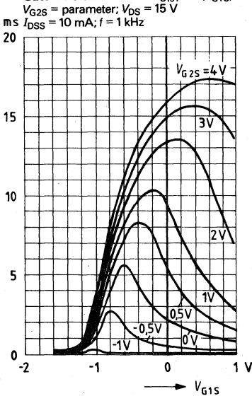
Gate 1 transmittance g_{fs1} = f(V_{G1S})
