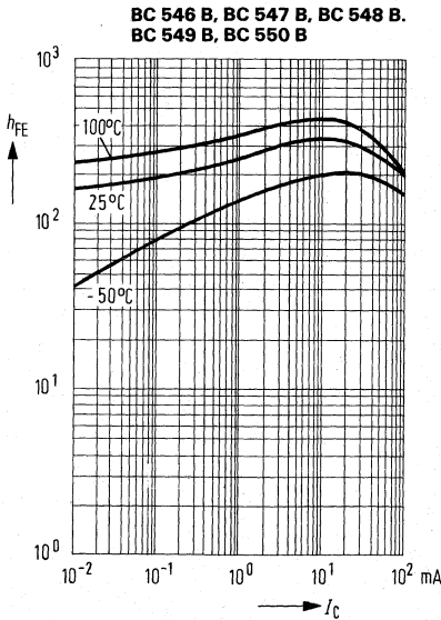
DC current gain h_{FE} = f(I_C) V_{CE} = 5 V ; T_{amb} = \text{parameter} (common-emitter configuration)
