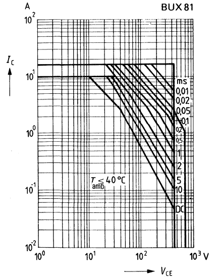
Permissible operating range I_C = f(V_{CE}); T_{amb} \leq 40^\circ\text{C}
