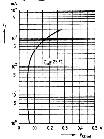
Collector-emitter saturation voltage V_{CEsat} = f(I_C) V_{CEsat} = f(I_C); h_{FE} = 10; T_{amb} = 25^\circ\text{C}
