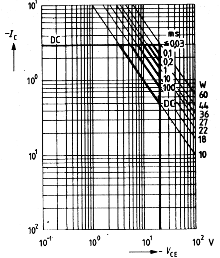
Permissible operating range I_C = f(V_{CE}) D = 0; T_{case} = 25^\circ C
