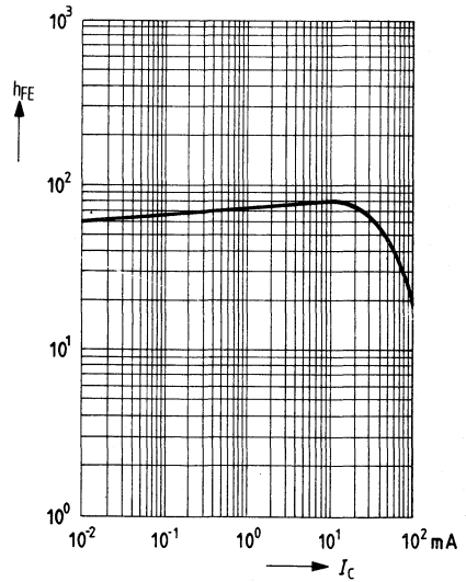
DC current gain h_{FE} = f(I_C) V_{CE} = 10 \text{ V}; T_{case} = 25 \text{ }^\circ\text{C}
