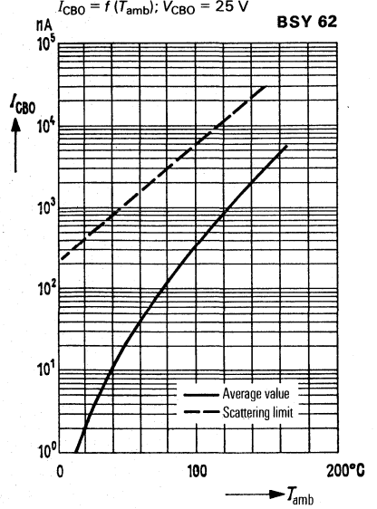
Collector cutoff current versus temperature I_{CBO} = f(T_{\text{amb}}); V_{CBO} = 25\text{ V}
