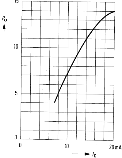
Output power P_o = f(I_C)
