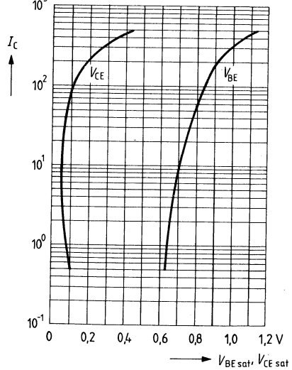
Saturation voltages
