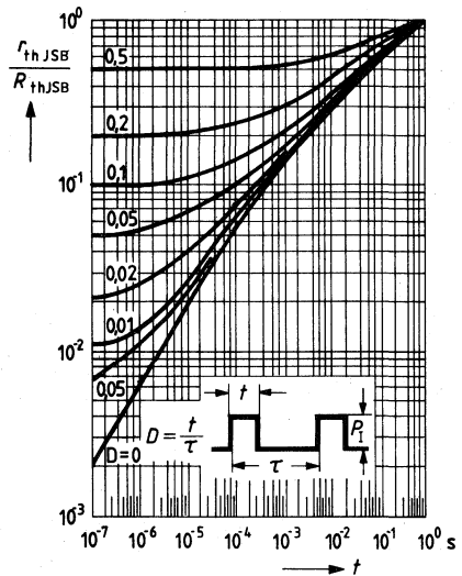
Perm. pulse load \frac{r_{thJSB}}{R_{thJSB}} = f(t)
