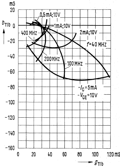
Small signal short circuit input admittance Y_{11b} (common base configuration)
