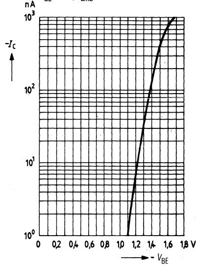
Collector current I_C = f(V_{BE}) V_{CE} = 2\text{ V}; T_{amb} = 25^{\circ}C
