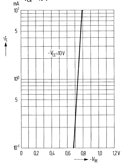
Input characteristic I_C = f(V_{BE}) -V_{CE} = 10\text{ V}
